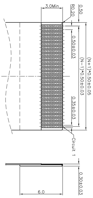
RECOMMENDED PFC/FTG DIMENSION
